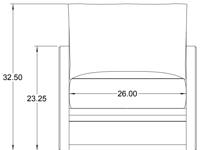
AVONDALE TEAK LOUNGE CHAIR 2960+FINISH
